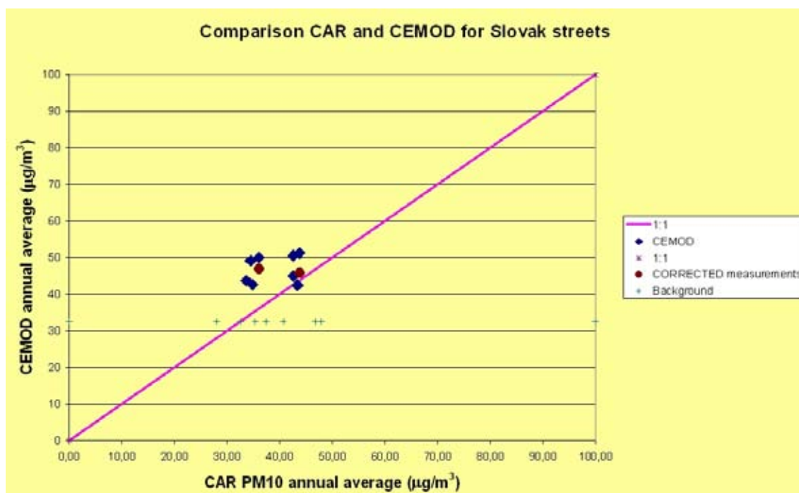
Obr. 4.1 Porovnanie modelov CAR a CEMOD pre \text{PM}_{10} .
