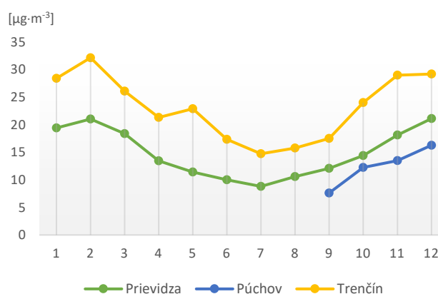
Fig. 3.6 Average monthly NO 2 concentrations.
