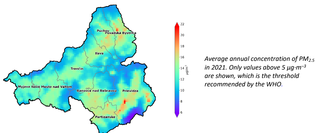
Fig. 3.5 Average annual PM 2.5 concentrations.
