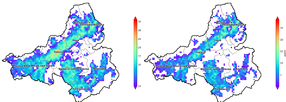
Fig. 3.3 Average annual PM_{10} concentration (left) and number of exceedances of the PM_{10} daily threshold (right) in 2021. Only values above 15 \mu g \cdot m^{-3} and non-zero number of exceedances are shown.
