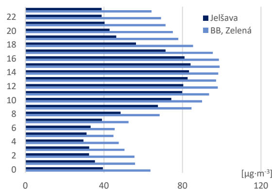
Fig. 3.10 Daily \text{O}_3 concentration in July 2022.
