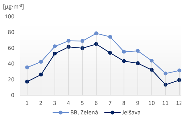
Fig. 3.8 Monthly average \text{O}_3 concentrations.
