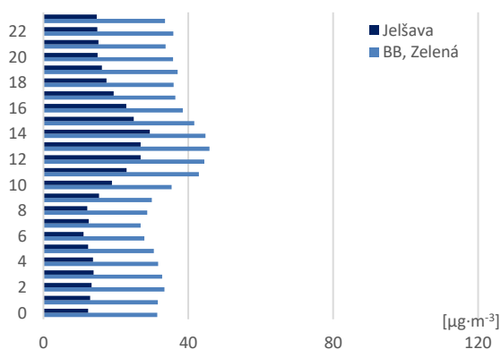
Fig. 3.9 Daily \text{O}_3 concentration in January 2022.
