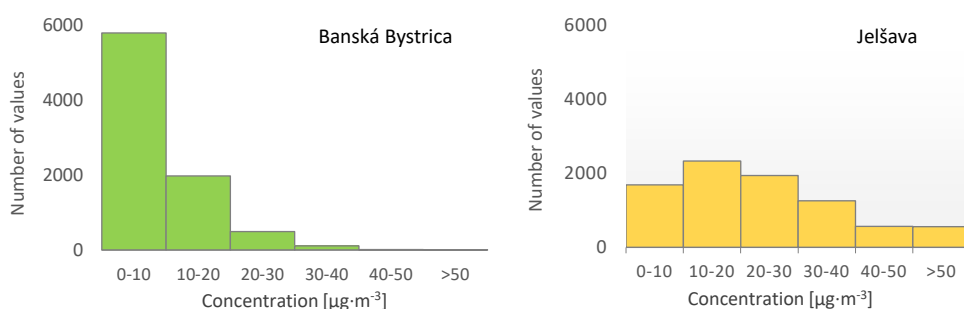
Fig. 3.7 Histogram of hourly \text{NO}_2 concentrations at AMS Banská Bystrica, Štefánikovo nábr. and Jelšava.
